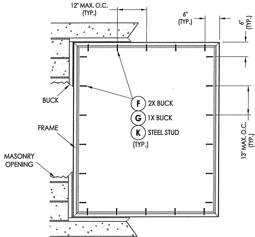
FRAME ANCHORING
