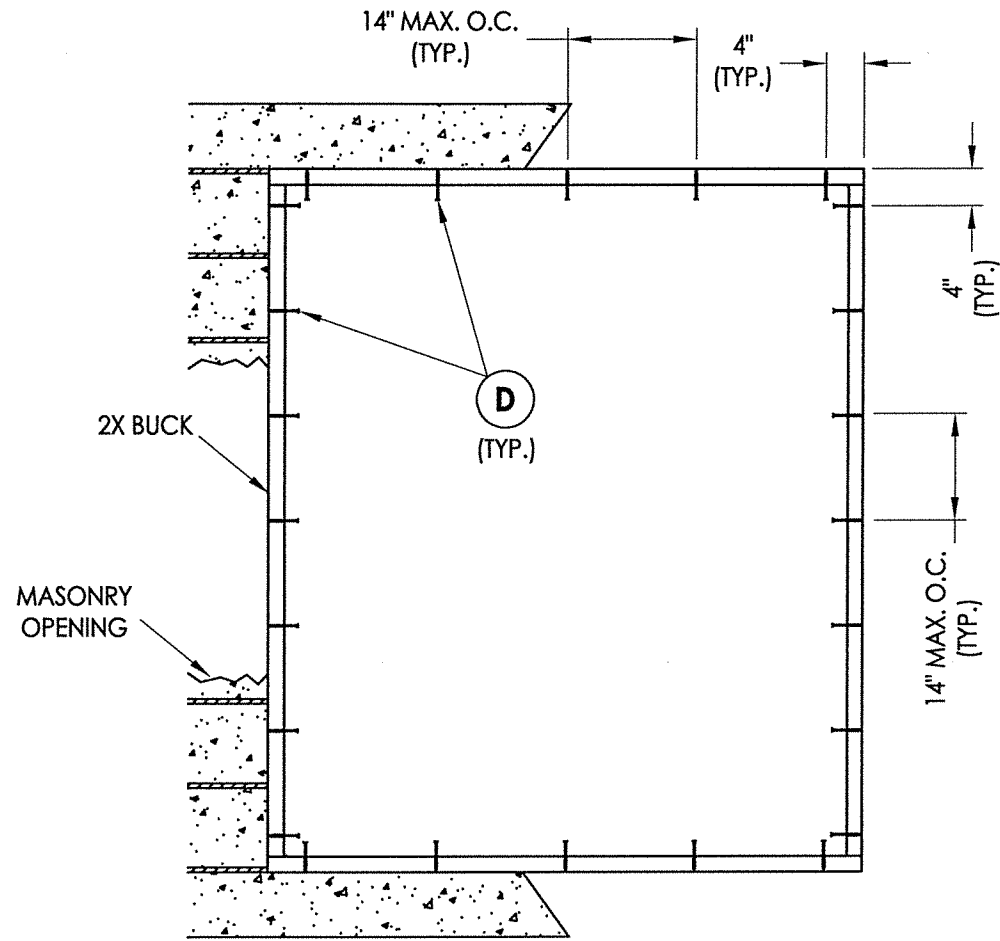
BUCK ANCHORING
